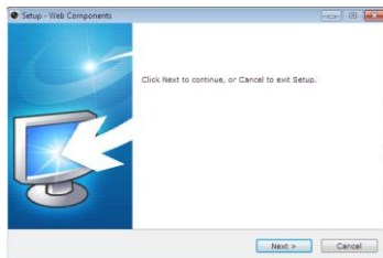
Figure 4-3 Instalace pluginu
