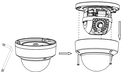
Figure 2-2 Demontujte kopuli
