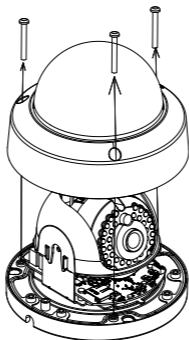
Figure 2-8 Demontáž kamery
