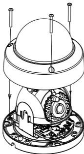
Figure 2-10 Nasadte kopuli
