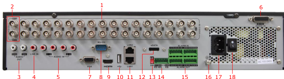
Figure 1.13 Rear Panel of DS-7332HFI-SH, DS-7332HWI-SH and DS-7332HI-SH
