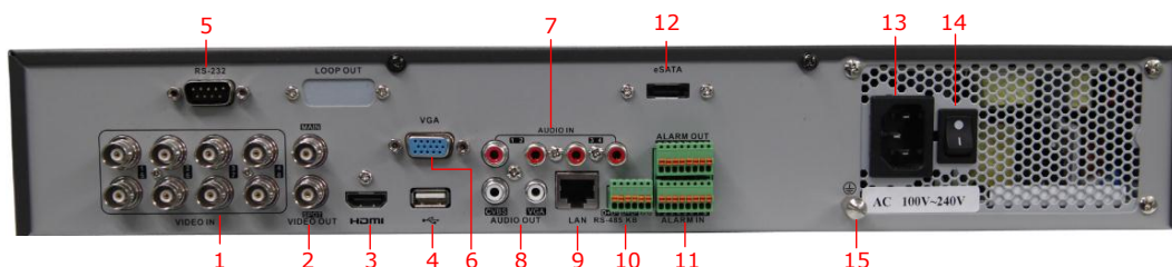
Figure 1.10 Rear Panel of DS-7308HFI-SH and DS-7308HWI-SH
