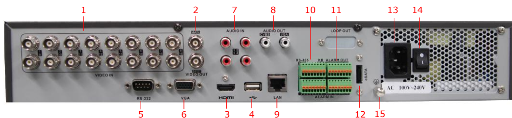
Figure 1.11 Rear Panel of DS-7316HFI-SH and DS-7316HWI-SH
