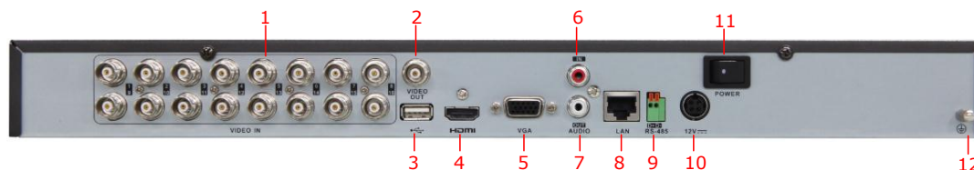
Figure 1.8 Rear Panel of DS-7216HFI-SH and DS-7216HWI-SH
