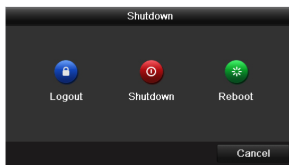
Figure 13.14 Shutdown Menu
