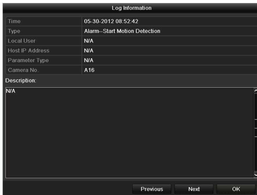
Figure 12.8 Log Details
