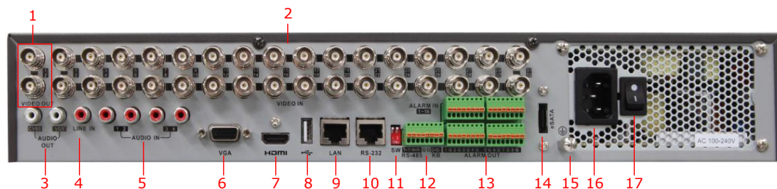
Figure 1.12 Rear Panel of DS-7332HFI-SH, DS-7332HWI-SH and DS-7332HI-SH
