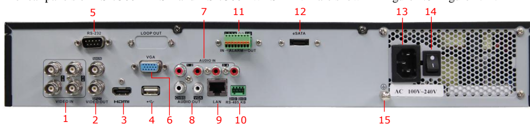
Figure 1.9 Rear Panel of DS-7304HFI-SH and DS-7304HWI-SH
