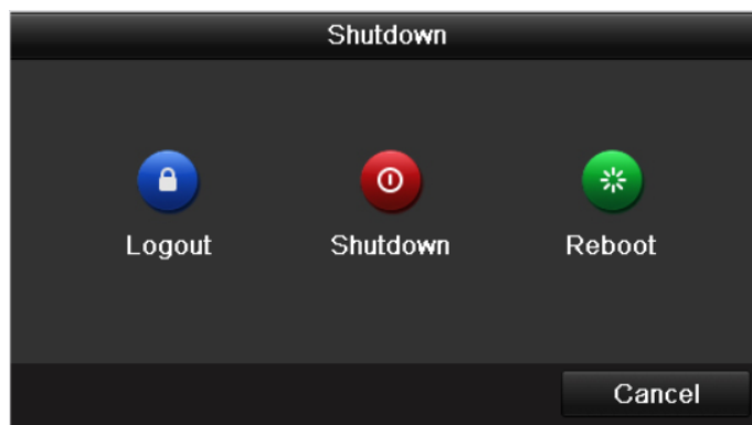
Figure 3.11 Shutdown
