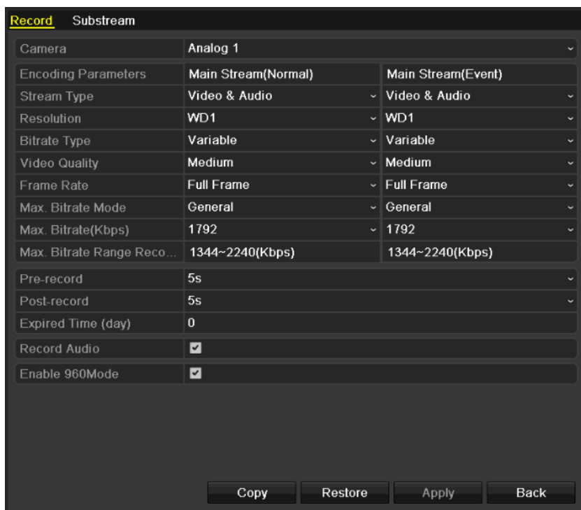
Figure 5.32 Encoding Record
